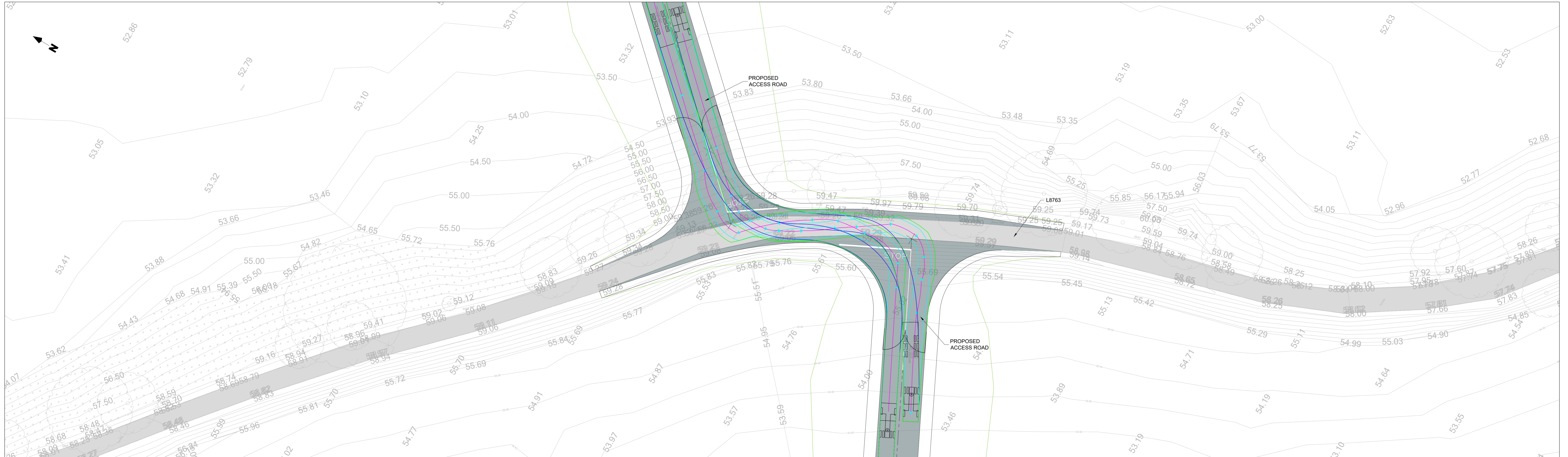
STAGGERED JUNCTION Scale 1:250
